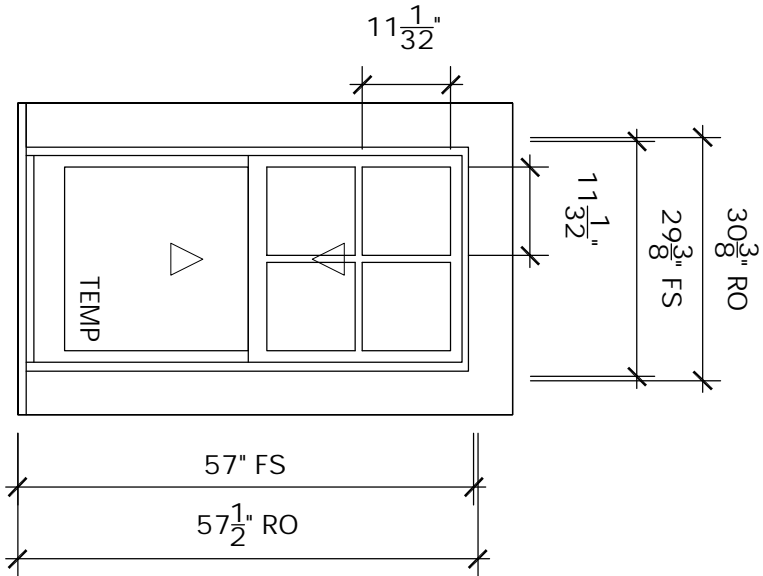
C QTY 3 WUDH 2424 SCALE: 1/2" = 1'-0" 6-9/16" JAMBS TEMPERED
